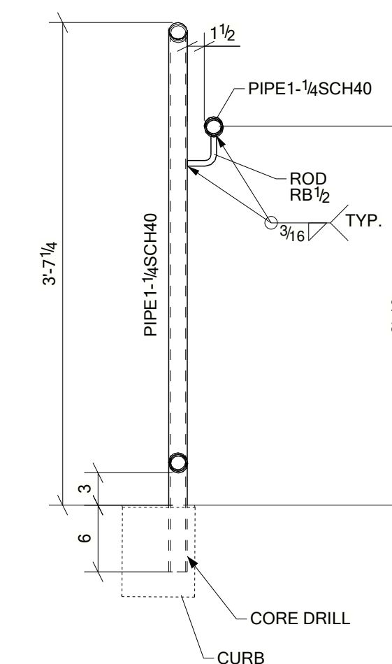
TYPICAL DETAIL
